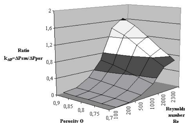
Figure 2 – The ratio of pressure drops in porous and smooth-walled steam generating channels k_{\Delta P} = \Delta P_{sm} / \Delta P_{por} ( T_{s0} = 110 °C; d = 4 mm; \Delta T = 4 °C)
