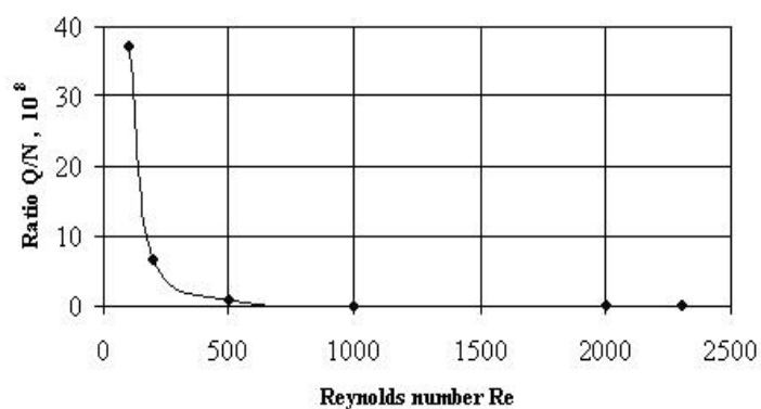
Figure 3 – Ratio of Q/N, 10^8 for a smooth-walled steam generating channel ( T_{s0}=110\text{ }^{\circ}\text{C} ; d=4\text{ mm} ; \Delta T=4^{\circ}\text{C} )
