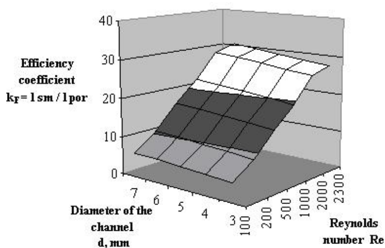
Figure 9 – The value of the geometric coefficient of efficiency of the porous steam generating channel k_F = l_{sm} / l_{por} = f(Re, d) ; ( T_{s0} = 110\text{ }^{\circ}\text{C} ; \Delta T = 4\text{ }^{\circ}\text{C} ; \Theta = 0,9 )
