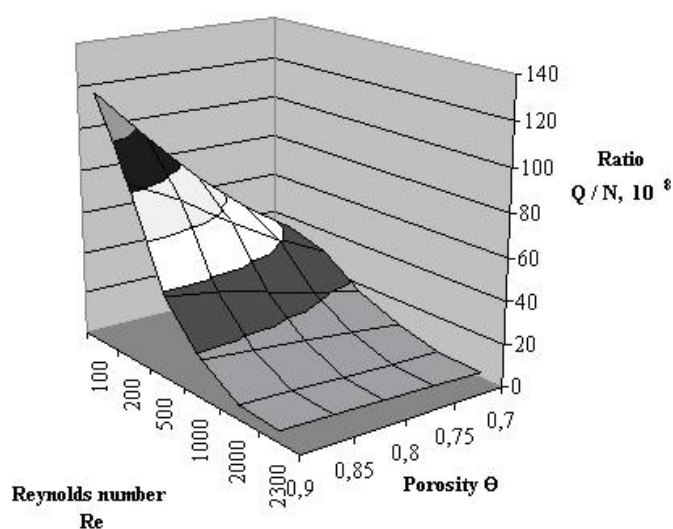
Figure 4 – Ratio of Q/N, 10^7 for a porous steam generating channel ( T_{s0}=110\text{ }^{\circ}\text{C} ; d=4\text{ mm} ; \Delta T=4^{\circ}\text{C} )
