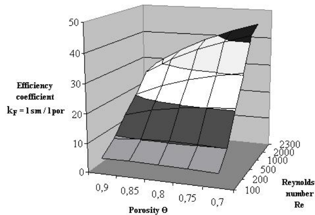
Figure 1 – The value of the geometric coefficient of efficiency of the porous steam generating channel k_F = l_{sm} / l_{por} ( T_{s0} = 110 °C; d = 4 mm; \Delta T = 4 °C)
